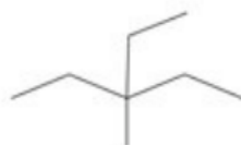
3-ethyl-3-methylpentane
