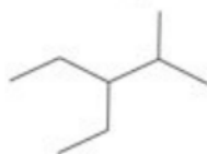
3-ethyl-2-methylpentane
